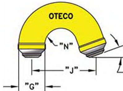
160° Standpipe Gooseneck (GSNK160)
