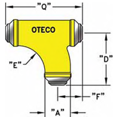
Long Sweep Tee (LST)
