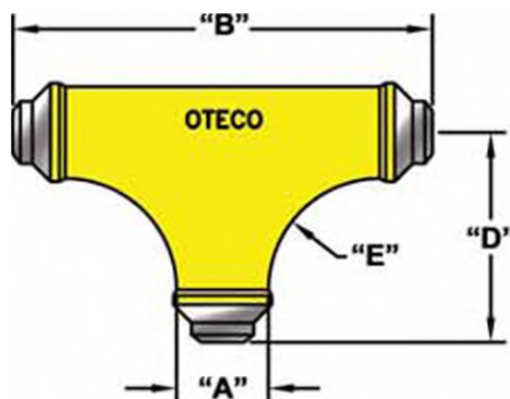
Long Sweep Full Flow Tee (LSFFT)
