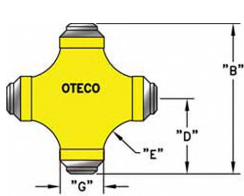
Full Flow Cross (FFC)
