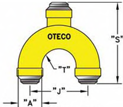
Long Sweep "Y" (LSY)
