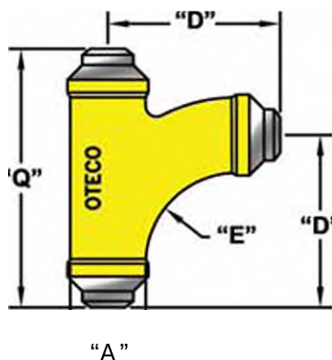
Long Sweep Tee (LST)
