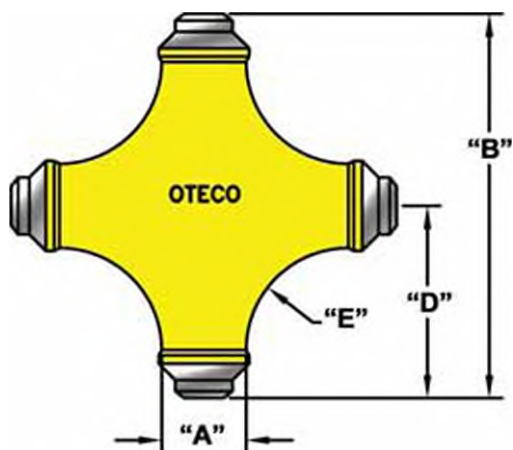
Long Sweep Full Flow Cross (FFC)
