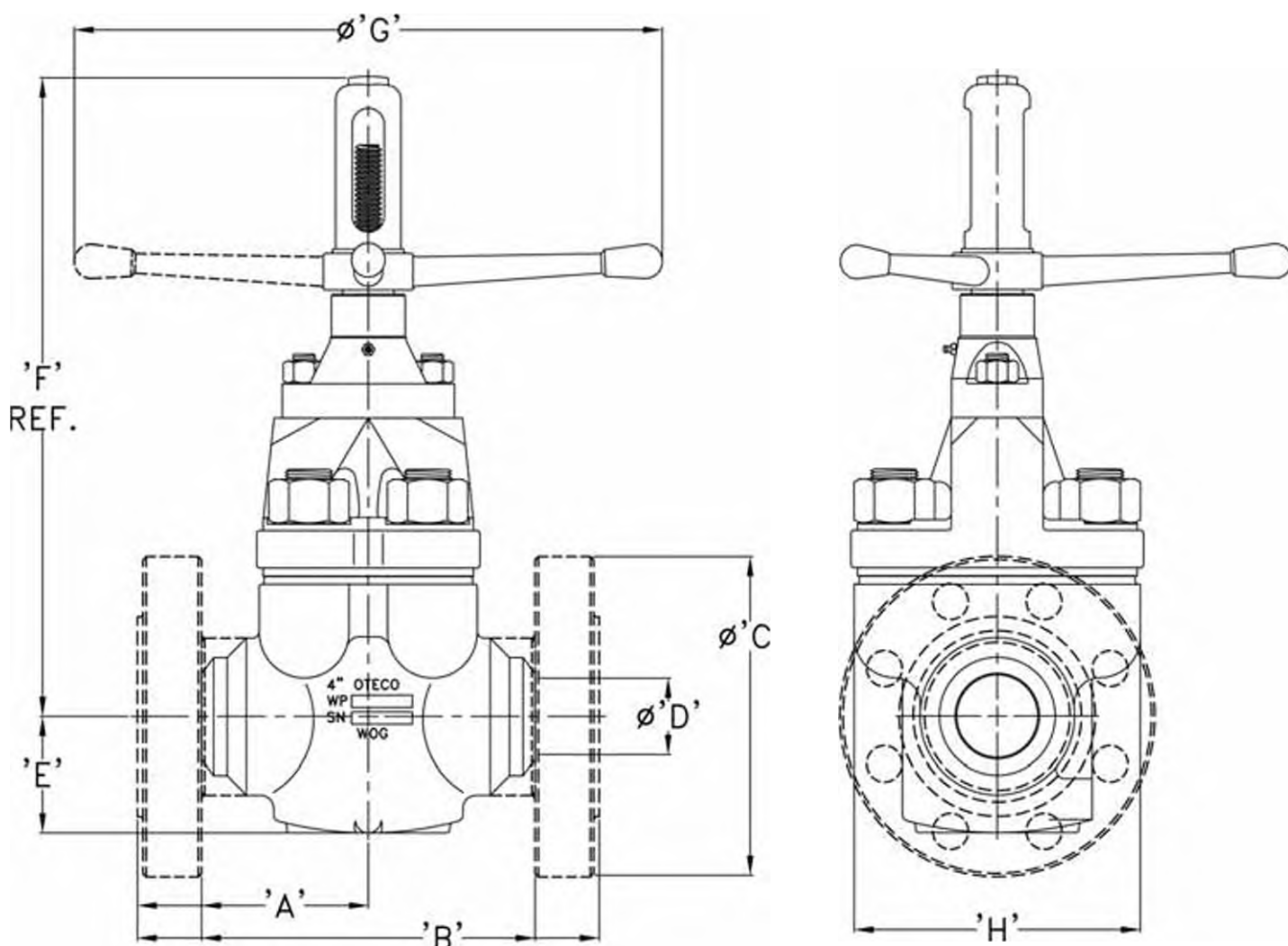
DM 45, 55, 48 & 58 SERIES GATE VALVE ASSEMBLIES - INCH (Metric mm)
